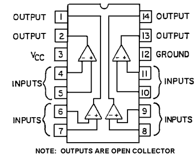
U4 & U5 19A704125P1 Quad Comparator
