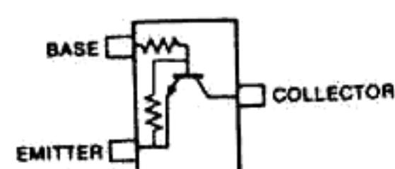
DTC144EU (Symbol: 26)
