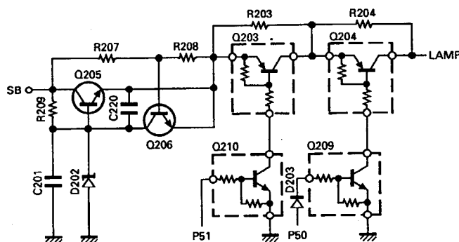
Fig. 8 Dimmer circuit
