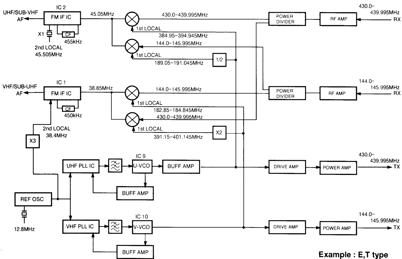
Fig.1 Frequency configuration
